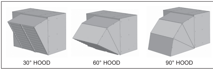
Figure 26.1 - 30°, 60°, & 90° Deflector Hoods
