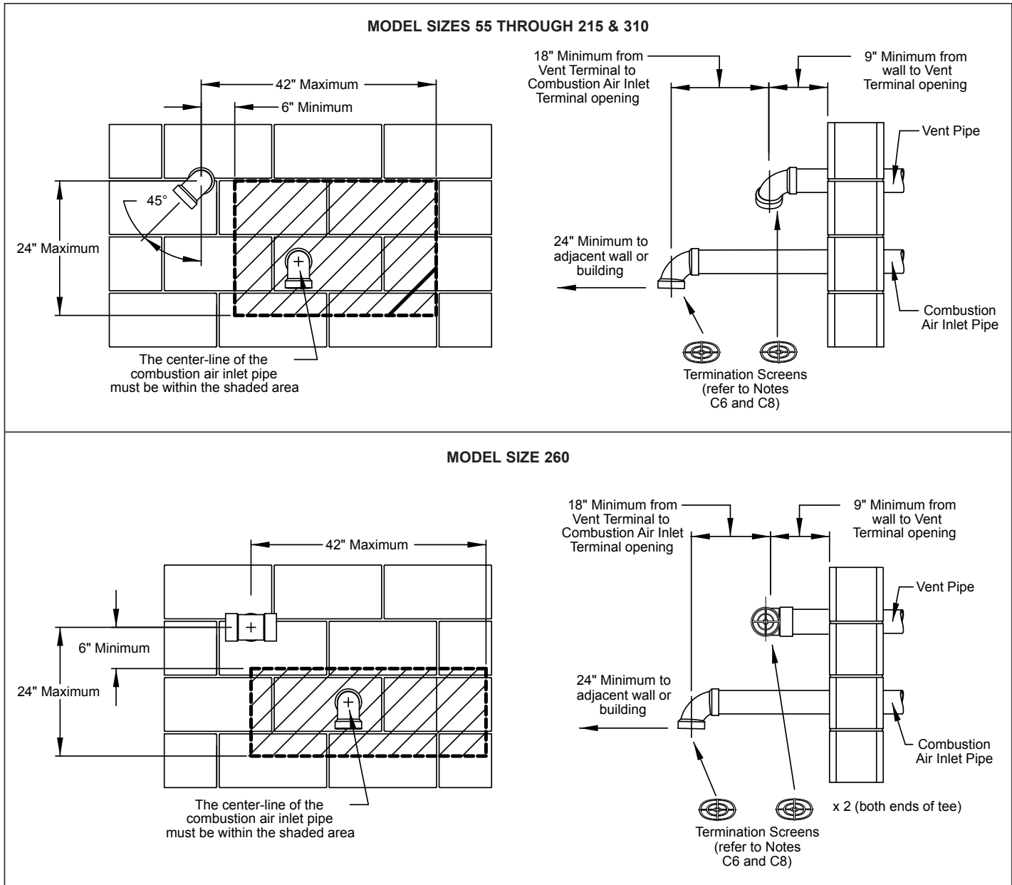
Figure 12.1 - Horizontal 2-Pipe Vent System
