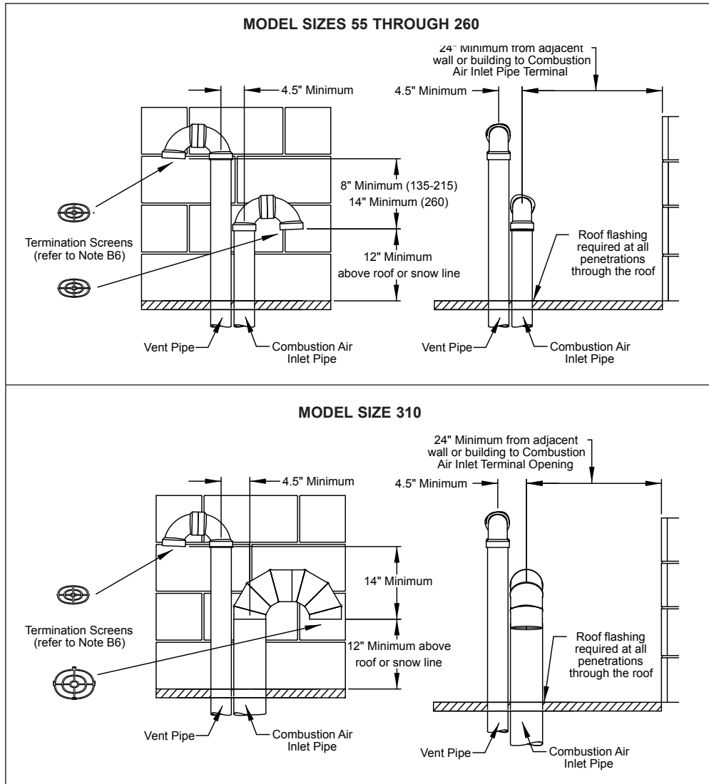
Figure 10.2 - Vertical 2-Pipe Vent System for Sloped Roofs
