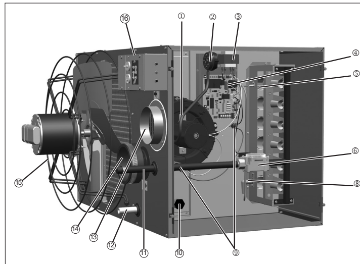
Figure 24.1 - Factory Mounted Standard Features
