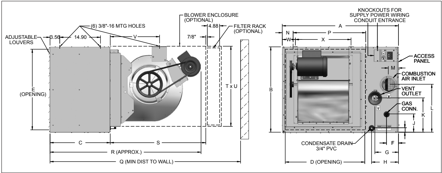
Figure 28.1 - Dimensional Drawings - Model BTC
