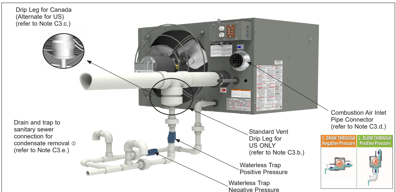
Figure 11.1 - Venting System Drip Leg and Condensate Drain Connections
