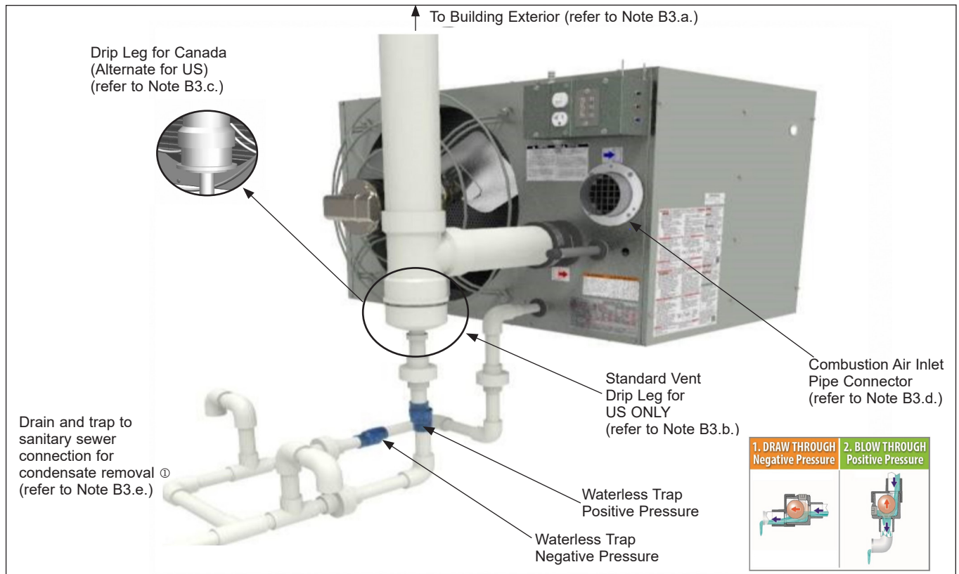
Figure 9.1 - Venting System Drip Leg and Condensate Drain Connections
