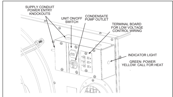
Figure 18.1 - Power/Control Wiring
