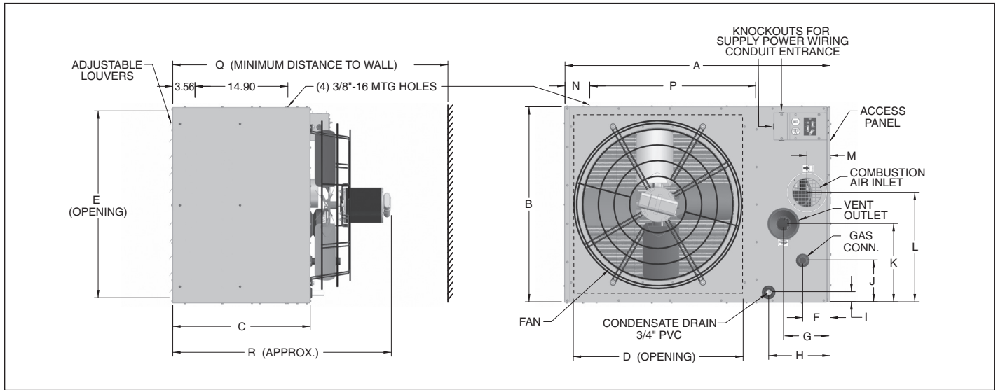
Figure 27.1 - Dimensional Drawings - Model PTC
