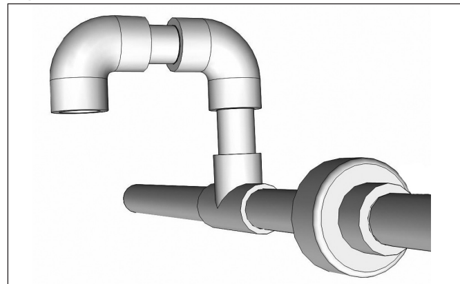
Figure 14.2 - Vacuum Breaker Example
