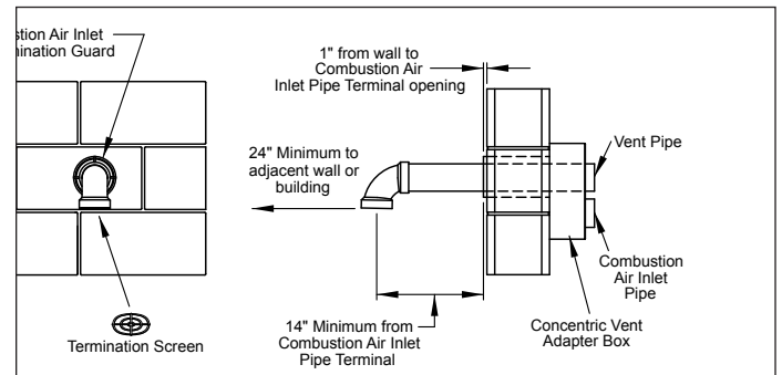
Figure 13.3 - Horizontal Concentric Vent Kit
