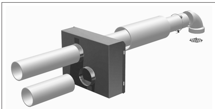
Figure 13.2 - Adapter Box Exploded Assembly
