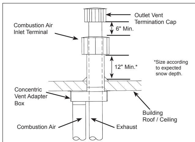
Figure 11.1 - Vertical Concentric Vent Kit Components
