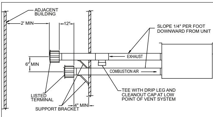
Figure 10.1 - Horizontal Venting with Downward Pitch
