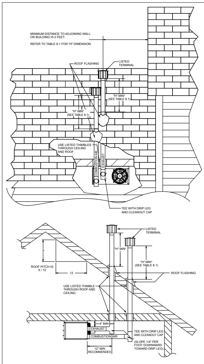
Figure 9.1 - Vertical 2-Pipe Vent System - Sloped Roof
