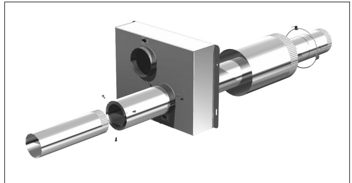
Figure 12.2 - Adapter Box Exploded Assembly
