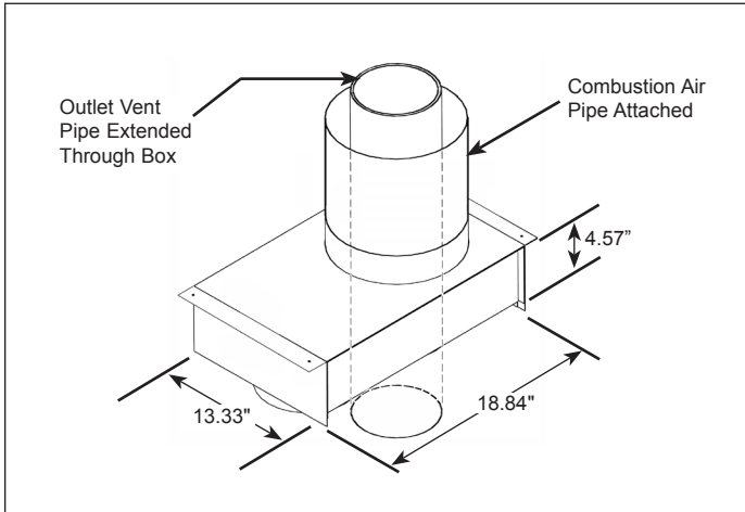
Figure 12.1 - Adapter Box with Combustion Air Intake Pipe Attached
