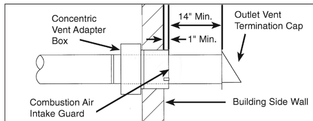
Figure 11.2 - Horizontal Concentric Vent Kit Components
