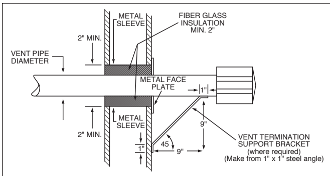
Figure 10.2 - Exhaust Vent Construction Through Combustible Walls and Support Bracket
