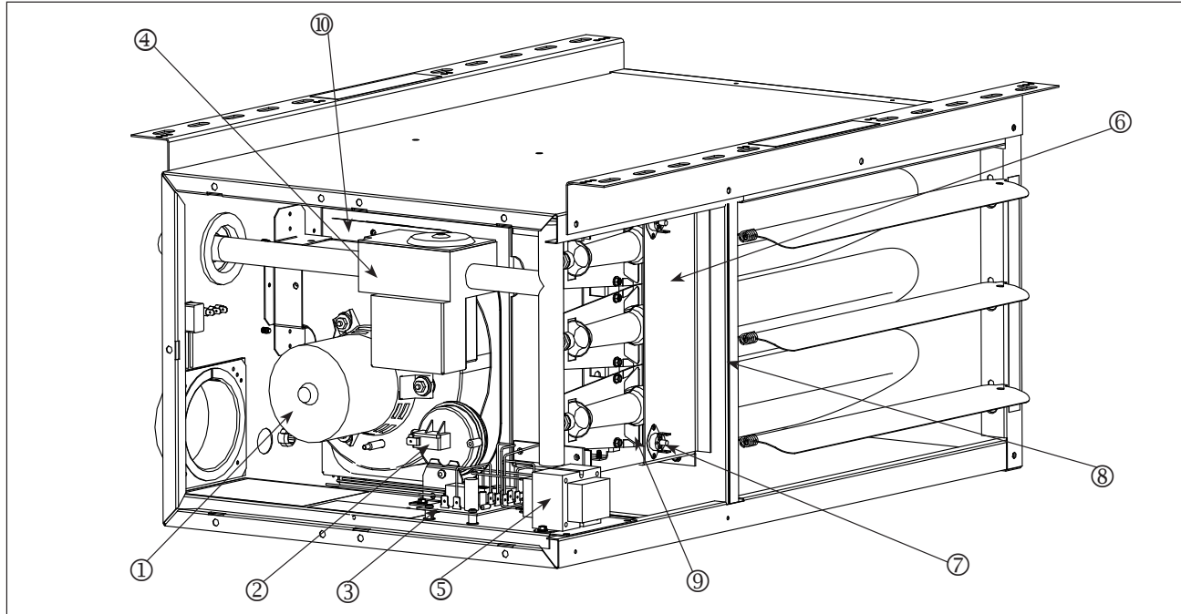
Figure 19.1 - Major Gas, Electrical Service, Safety and Other Components
