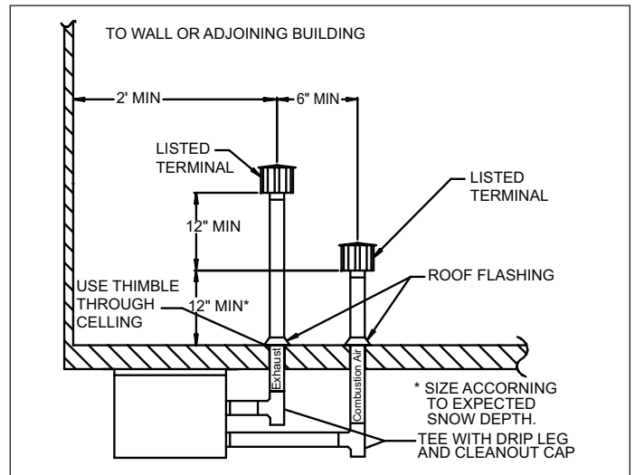
Figure 9.2 - Vertical 2-Pipe Vent System - Flat Roof
