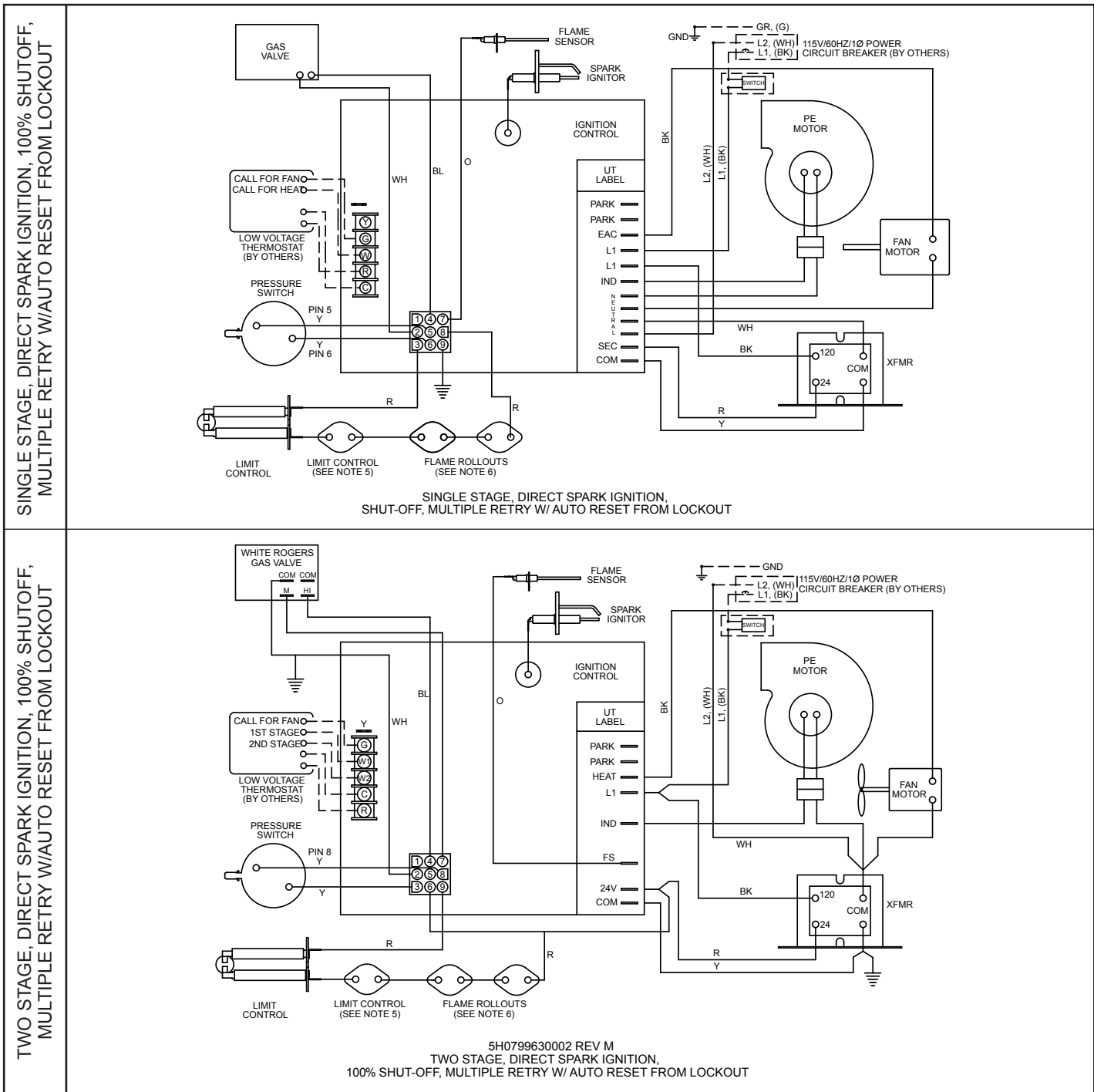
Figure 22.1 - Unit Heater Wiring Diagram (Single and Two Stage, Direct Spark Ignition)
